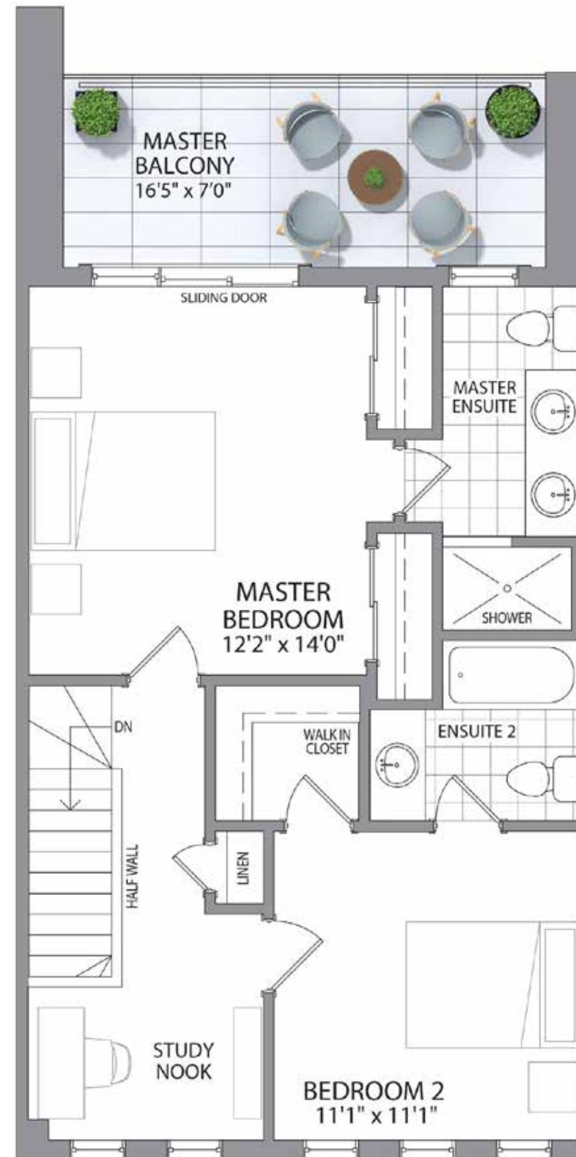
Third Floor
