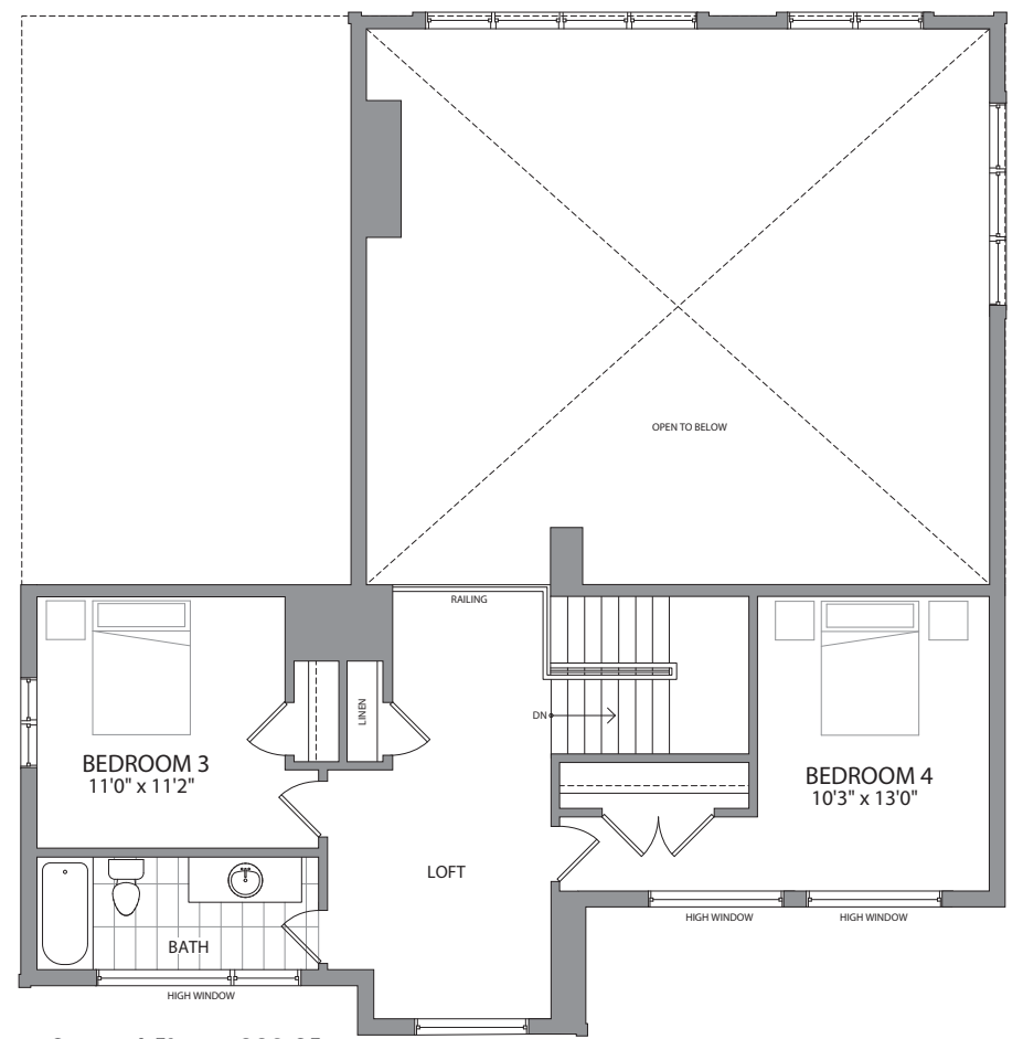
Second Floor- 662 SF Elevation A
